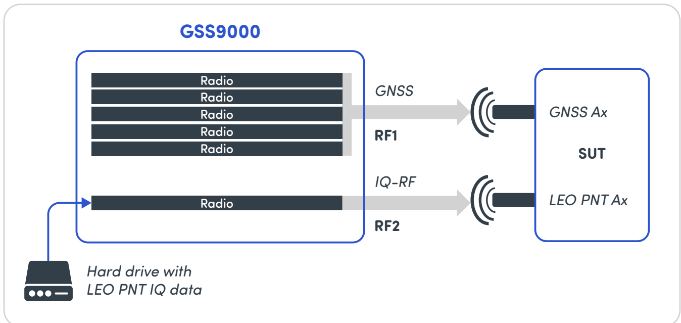
Interoperability testing—dual RF simulator employing SimIQ Replay
